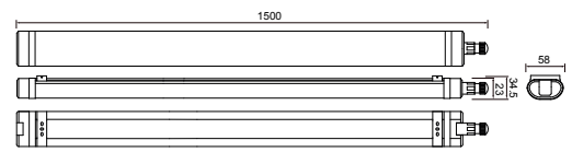
LD-HOU45W15-NB
